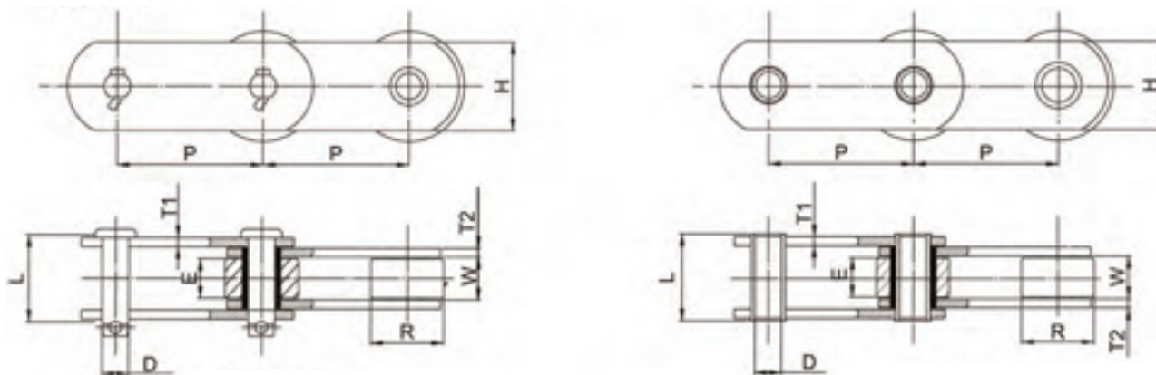
Solid Pin Type
