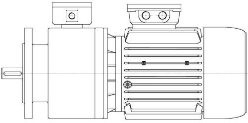
Standard B5 motor + VIS brake
